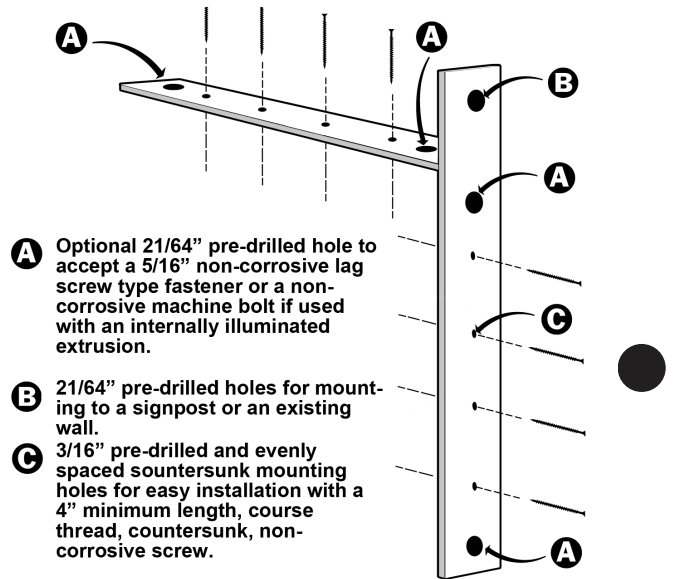
WALL MOUNT PROJECTION
